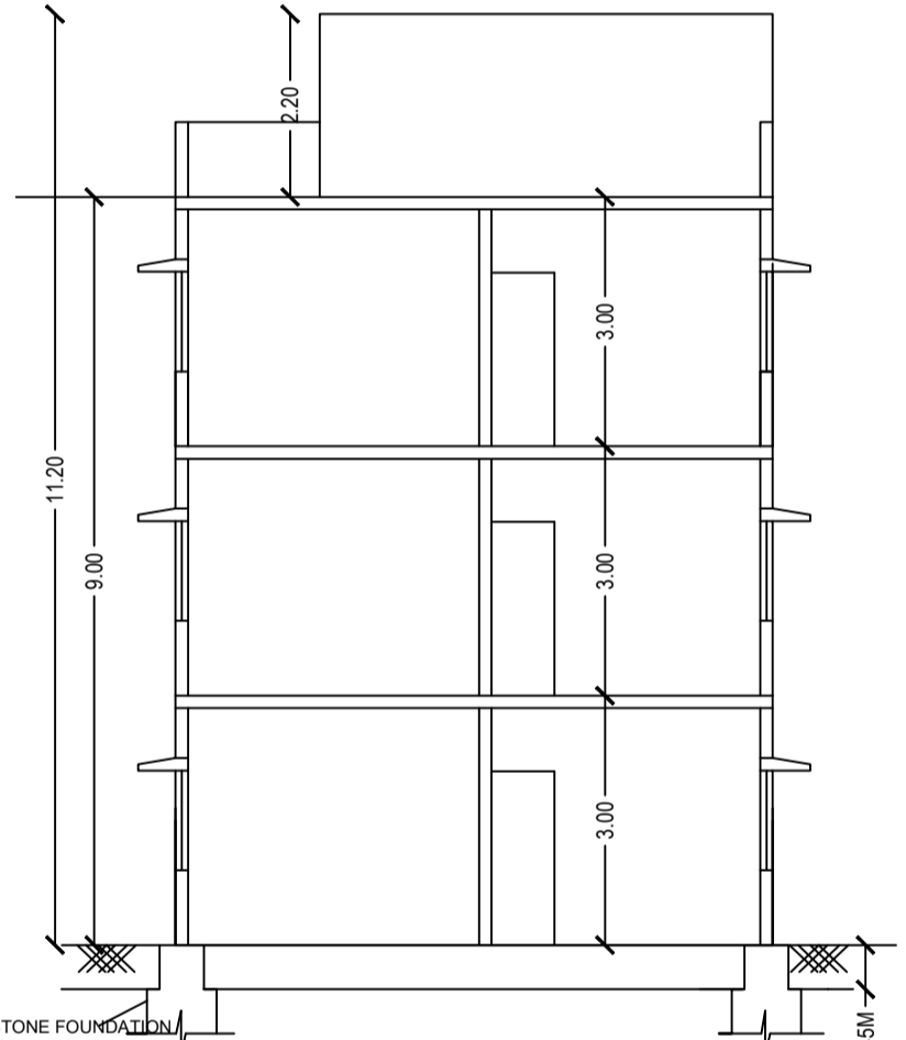
SECTION AT-XX
